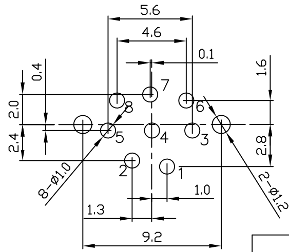
P.C.B. LAYOUT(±0.1) (TOP VIEW)
